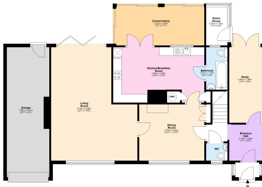
Ground Floor Approx. 121.2 sq. metres (1304.3 sq. feet)
